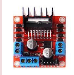
L298N Motor Driver
