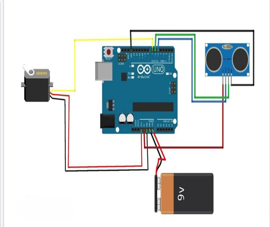
Automatic Dustbin
