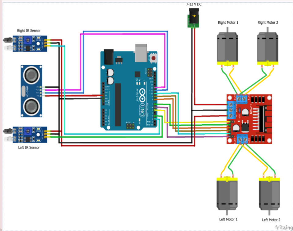
Human following car
